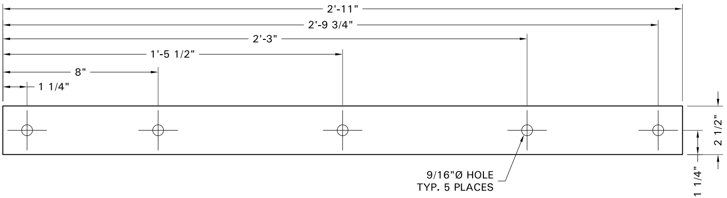
5HS-22 5 HOLE STRAP 2 1/2" x 2'-11" x 3/16" STAINLESS STEEL PLATE
