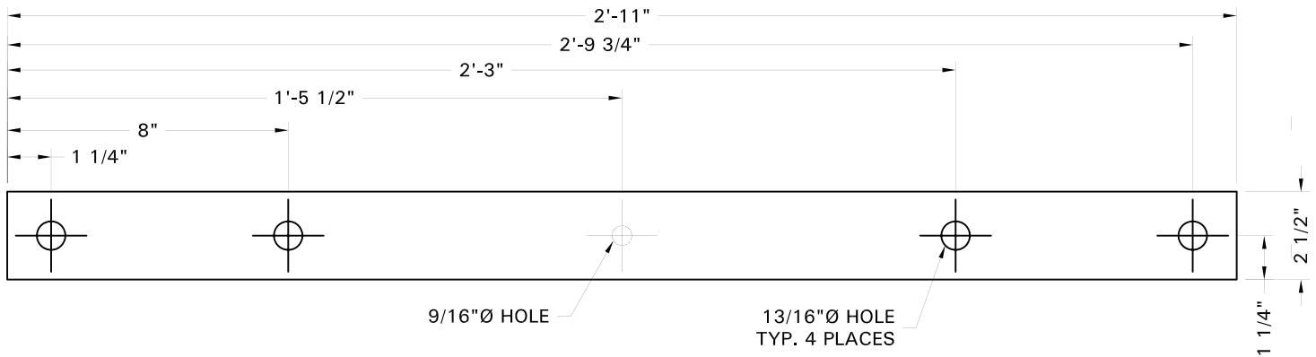
5HS-24 5 HOLE STRAP 2 1/2" x 2'-11" x 3/16" STAINLESS STEEL PLATE QTY. ( )
